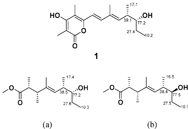
Figure 2. Comparison of 13 C NMR chemical shifts (in CDCl 3 ) of salinipyronone A ( 1 ) with two synthetic model compounds (a and b) to establish the relative configurations at C-10 and C-11 in 1 .
