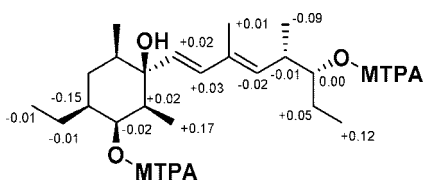
Figure 6. 1 H NMR \Delta\delta_{S-R} values in ppm for the bis- S - and R -MTPA esters of alcohol 5 in CD 3 OD.
